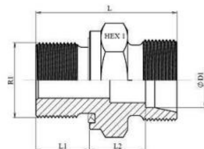
Selection Table : Straight Male BSP Parallel Union with seal S (Heavy) Series - Steel
