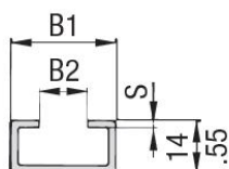
Mounting Rail TS-14
