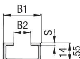
Mounting Rail TS-14
