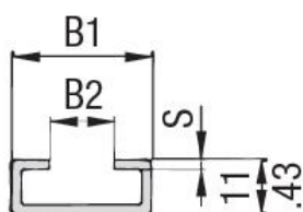
Mounting Rail TS-11
