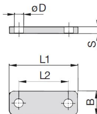
Selection Table : Cover Plate Heavy Series - Stainless Steel 1.4571 AISI 316 Ti
