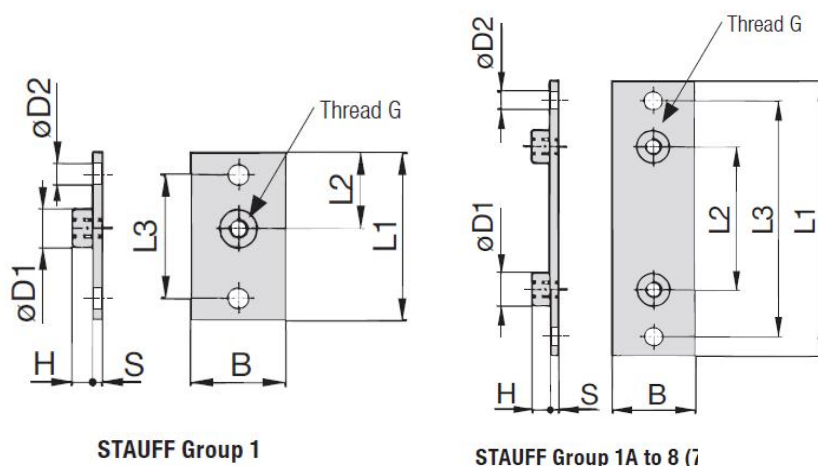
Selection Table : Standard series Elongated Weld Plate – Stainless Steel 1.4571 AISI 316 Ti
