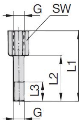
Selection Table : Threaded intermediate screw – Heavy series phosphated steel
