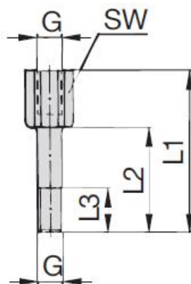
Selection Table : Intermediate Threaded Stacking Bolts Twin Series – Zinc/Nickel-Coated Steel
