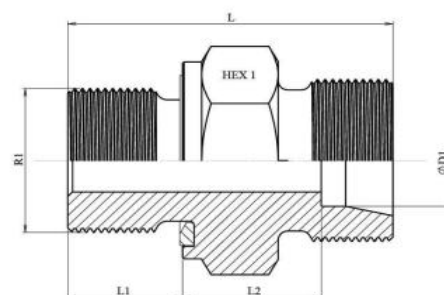
Selection Table : Straight Male Metric Parallel Union with seal L (Light) Series - Steel
