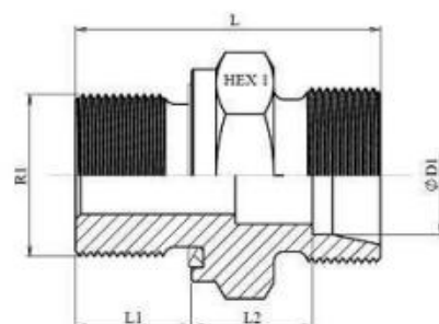
Selection Table : Straight Male BSP Parallel Union with seal L (Light) Series - Steel
