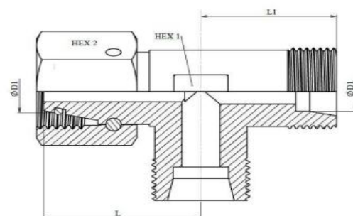
Selection Table : Reversed Adjustable Tee Male/Male/Female L (Light) Series - Steel
