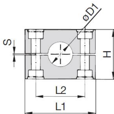
Selection Table : Clamp Body Heavy Series Profiled - Polypropylene
