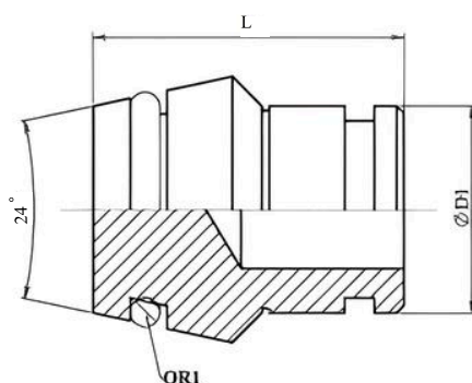
Selection Table : Closing Plug with o'ring L (Light) Series - Steel
