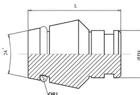
Selection Table : Closing Plug with o'ring L (Light) Series - Steel
