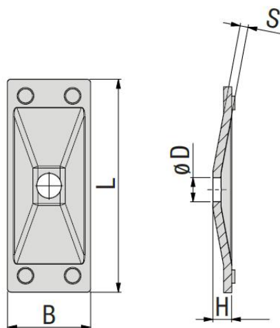
Selection Table : Protection plate – Double series zinc/nickel coated steel
