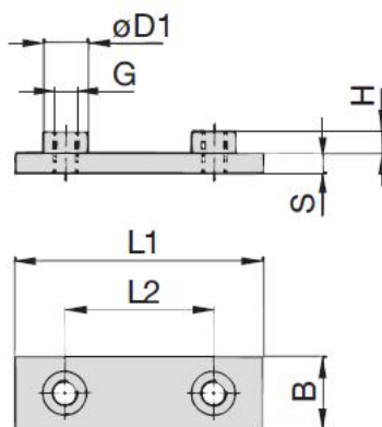
Selection Table : Weld Plate Heavy Series - Stainless Steel 1.4571 AISI 316 Ti
