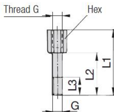
Selection Table : Standard Series Threaded intermediate screw – Stainless Steel 1.4571 AISI 316 Ti
