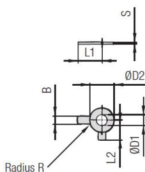
Safety Washer SI
