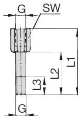
Selection Table : Intermediate threaded screws Twin Series - Stainless Steel 1.4571 AISI 316 Ti
